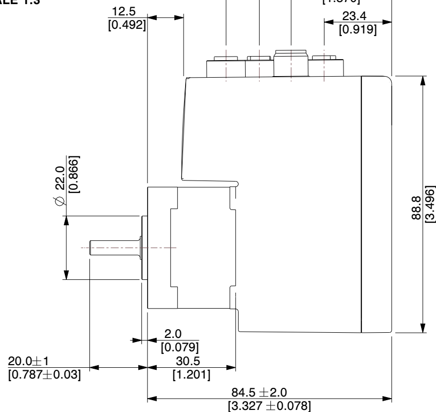
SHAFT DETAILS SCALE 1.3
